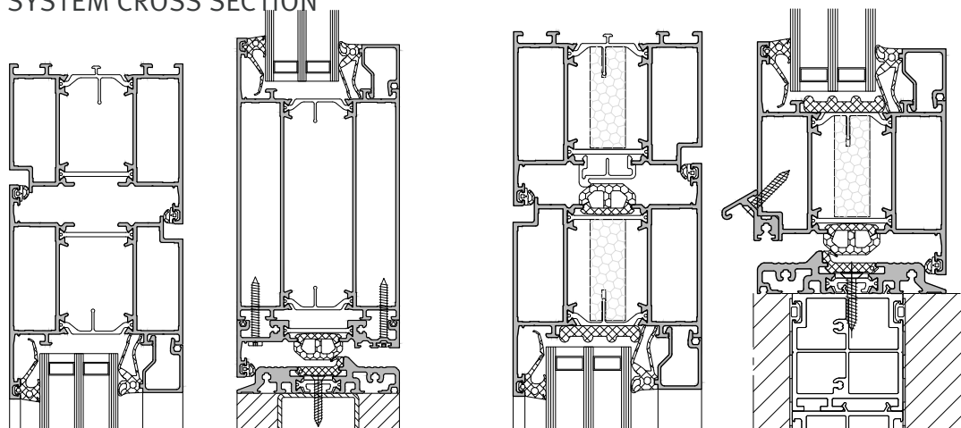
thermally insulated
