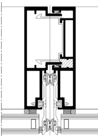
Mullion
