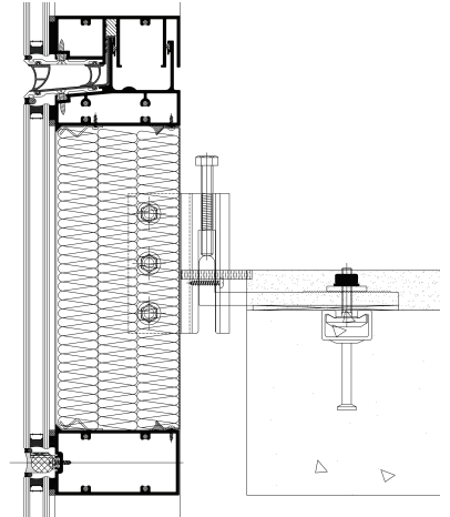
Bracket and Hooking System
