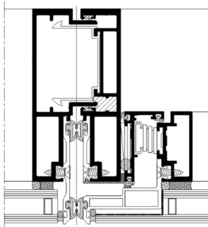
Mullion with Operable
