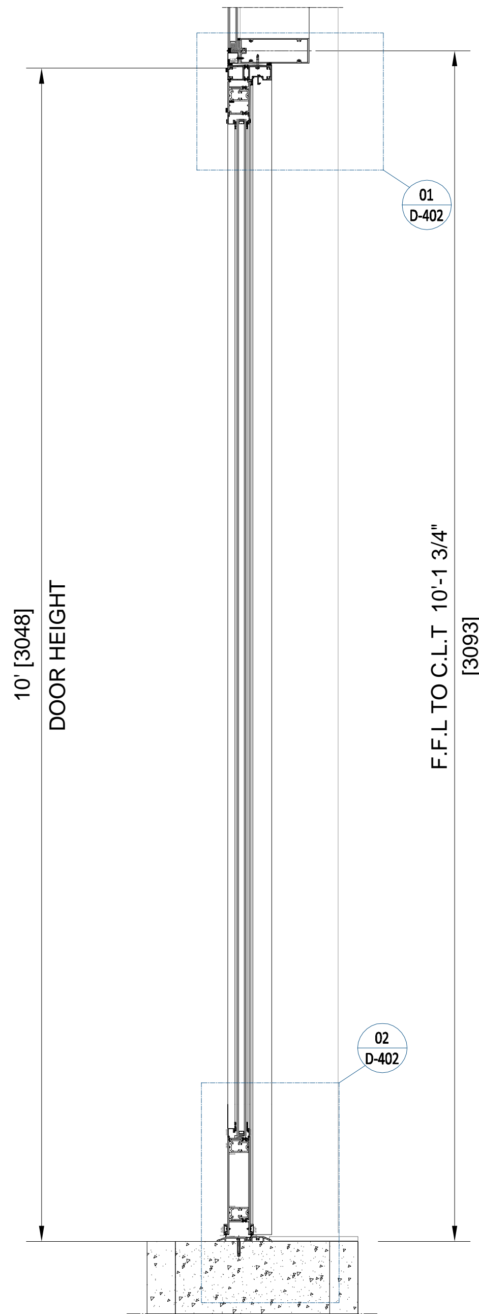
02 D-202 SECTION Scale - 1:10
