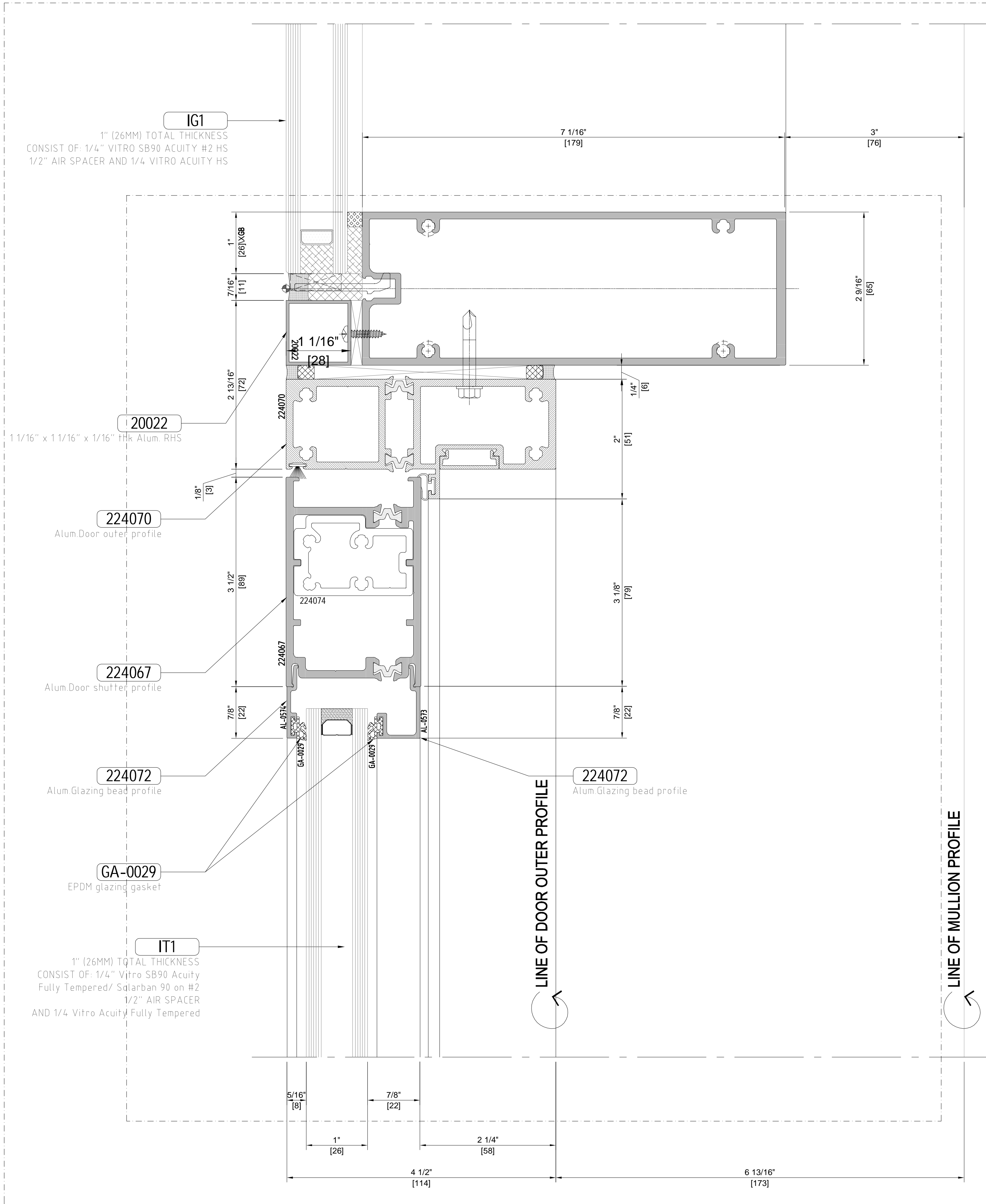
01 D-402 Vertical detail Scale: 1:1
