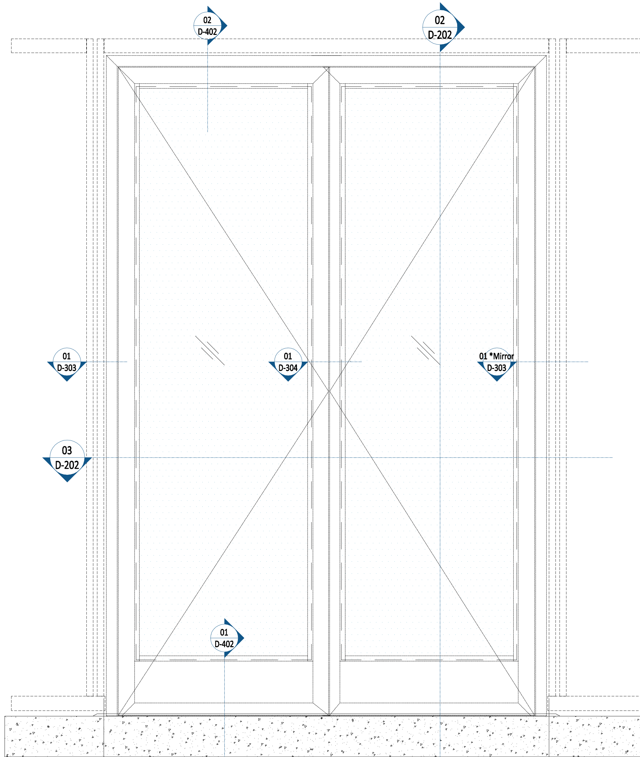
6'-8 7/8" [2054] CLEAR OPENING ELEVATION 01 D-202 Scale - 1:10
