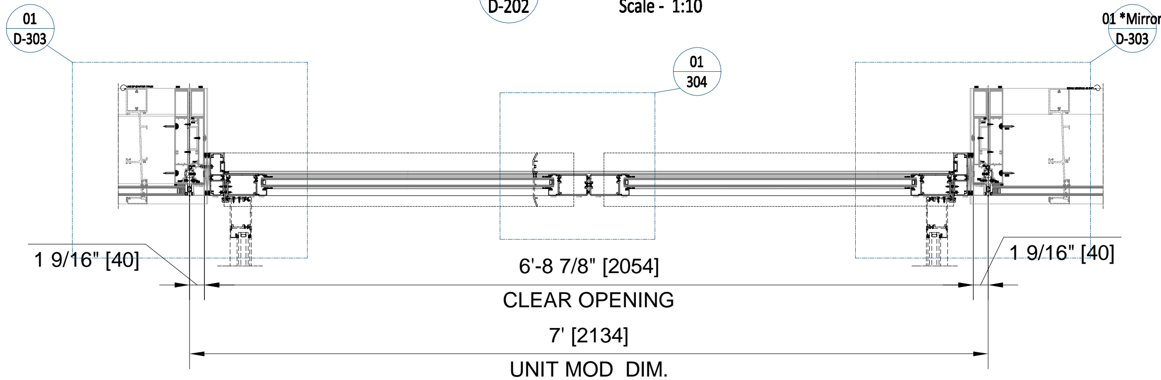
6'-8 7/8" [2054] CLEAR OPENING ELEVATION 01 D-202 Scale - 1:10
