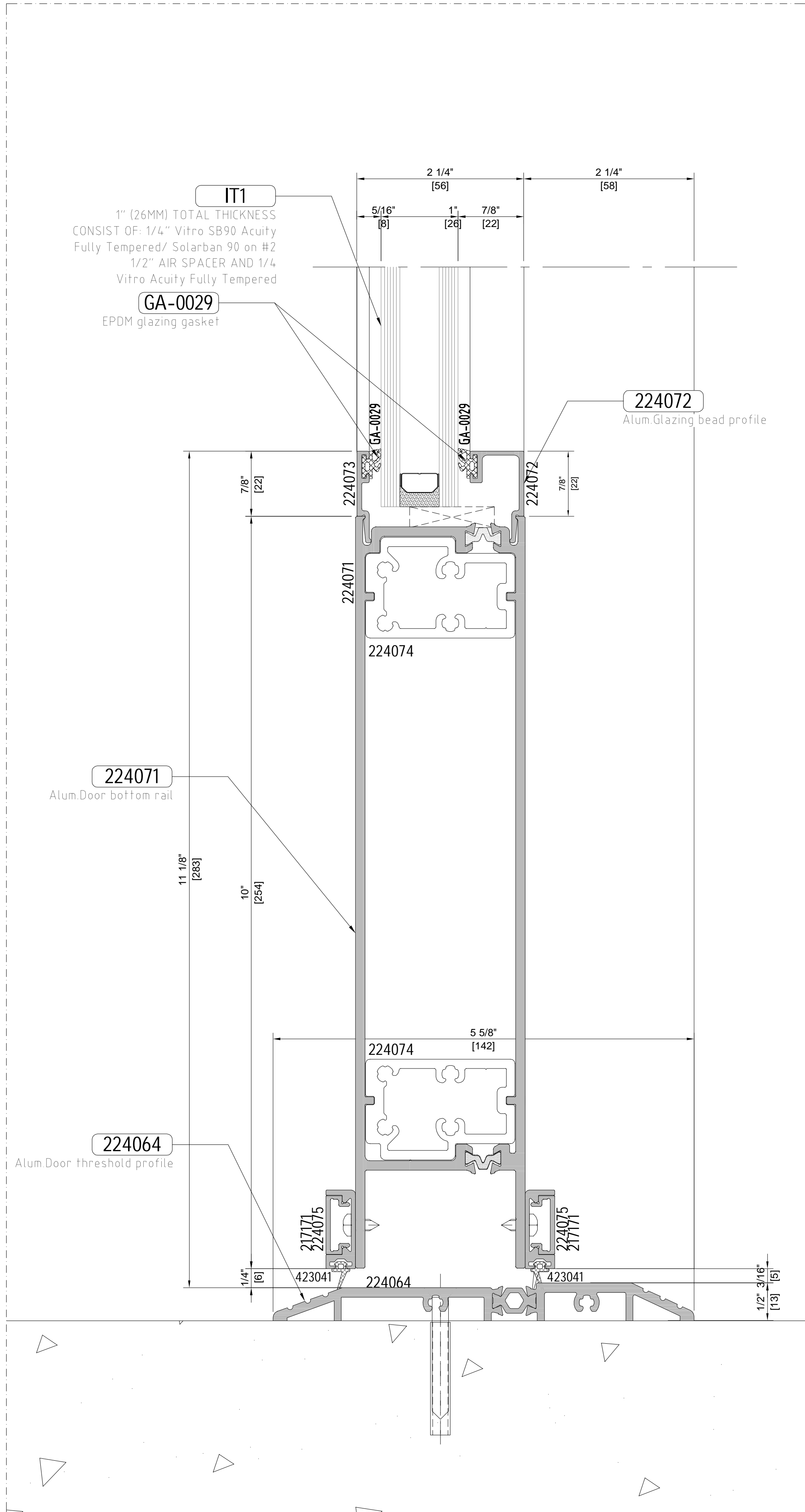
02 D-402 Vertical detail Scale: 1:1
