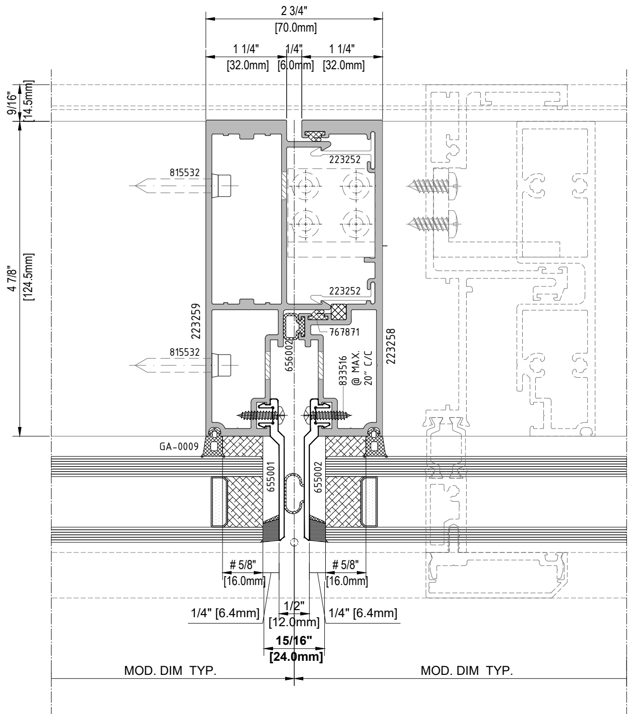
02 SECTION DETAIL
