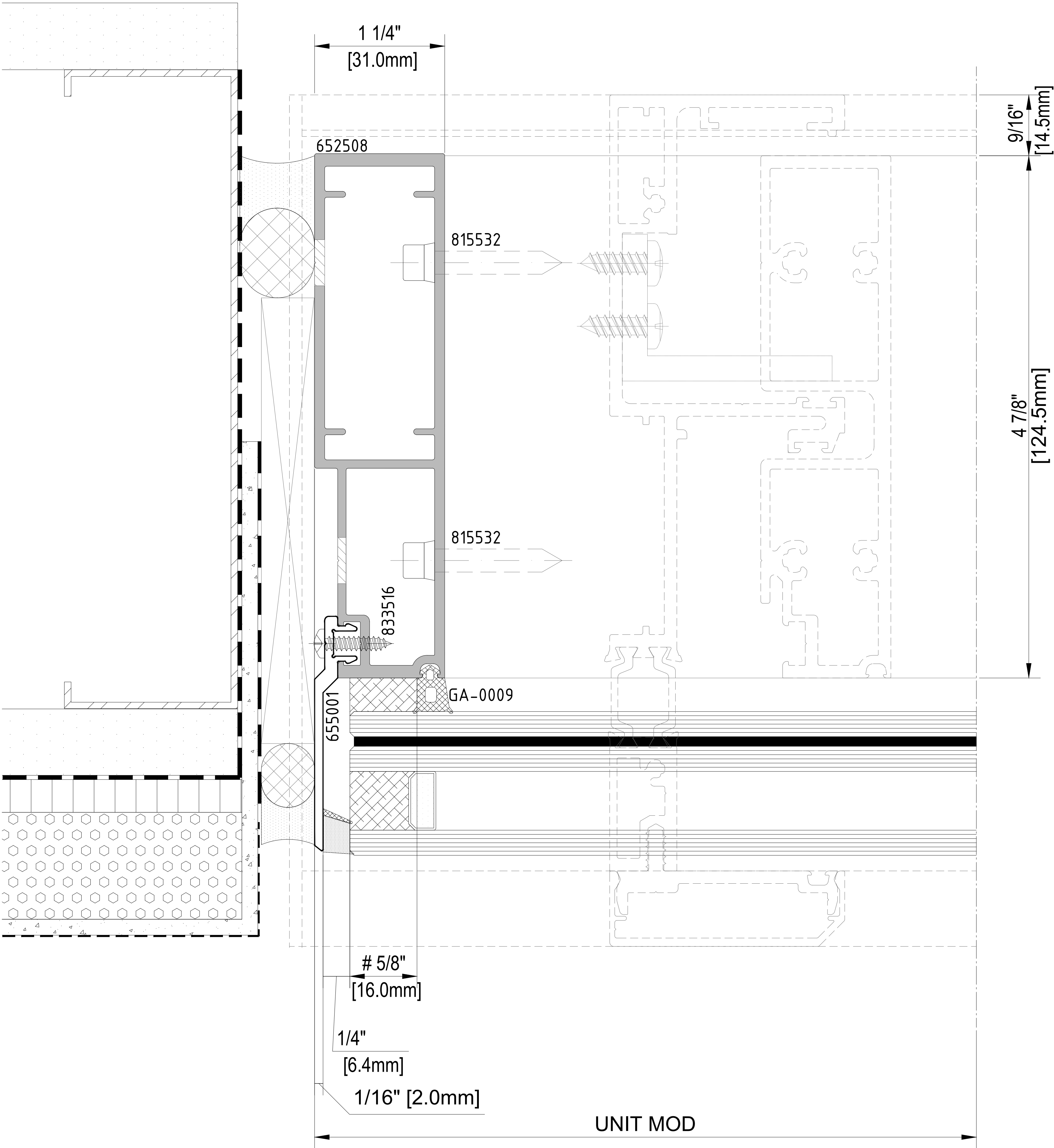
01 SECTION DETAIL
