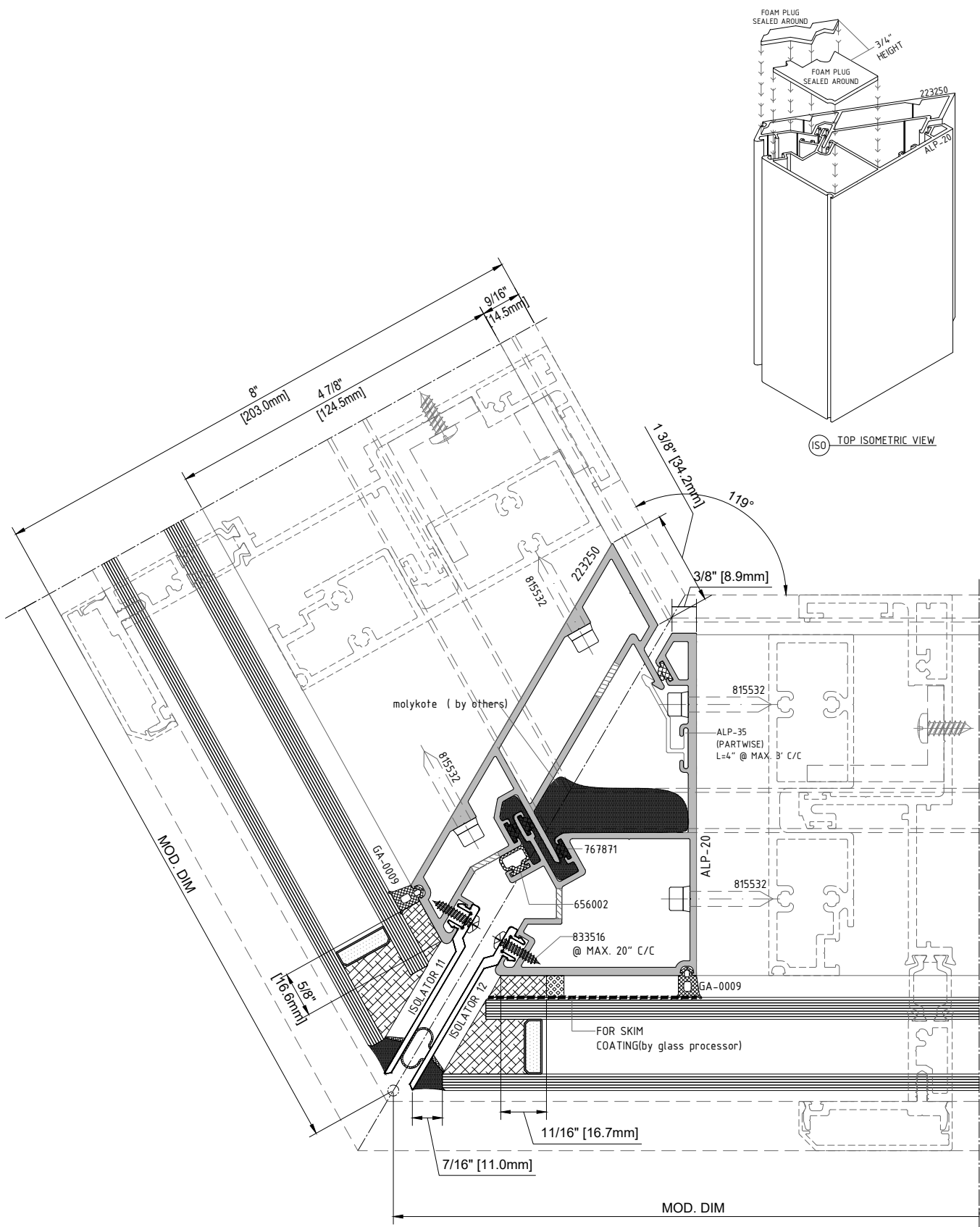
06 SECTION DETAIL
